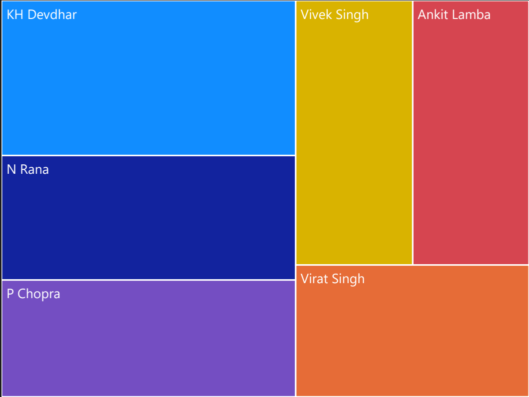
Dot Balls Played by Batters
