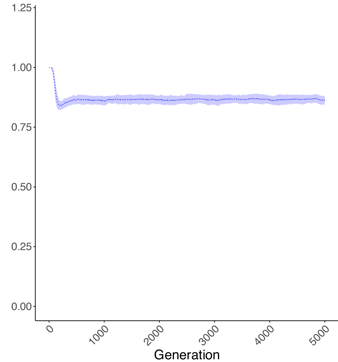
Insertion Bias = 50
