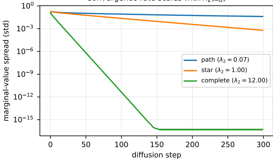
Convergence rate scales with \lambda_2(L_G)
