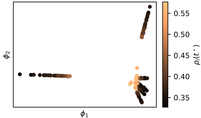
Heat residual on diffusion map
