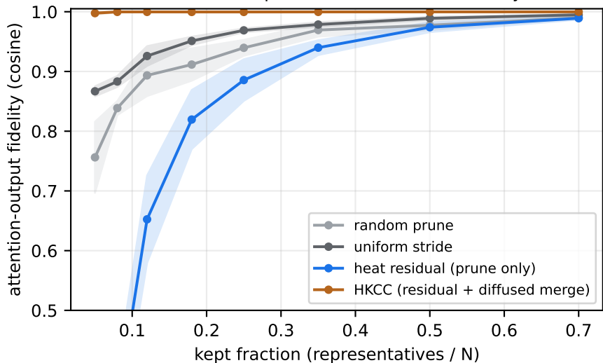
Context compression vs. attention fidelity
