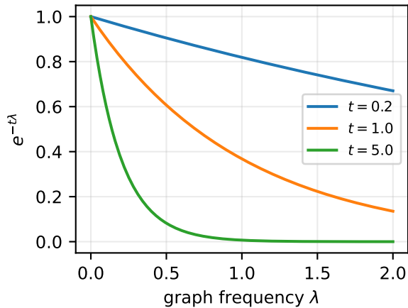
(b) heat kernel = low-pass
