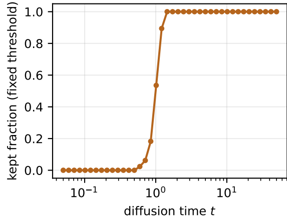
(a) the compression dial
