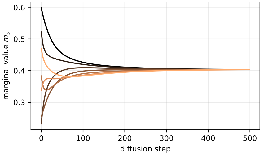
Budget-as-heat: marginals equalize
