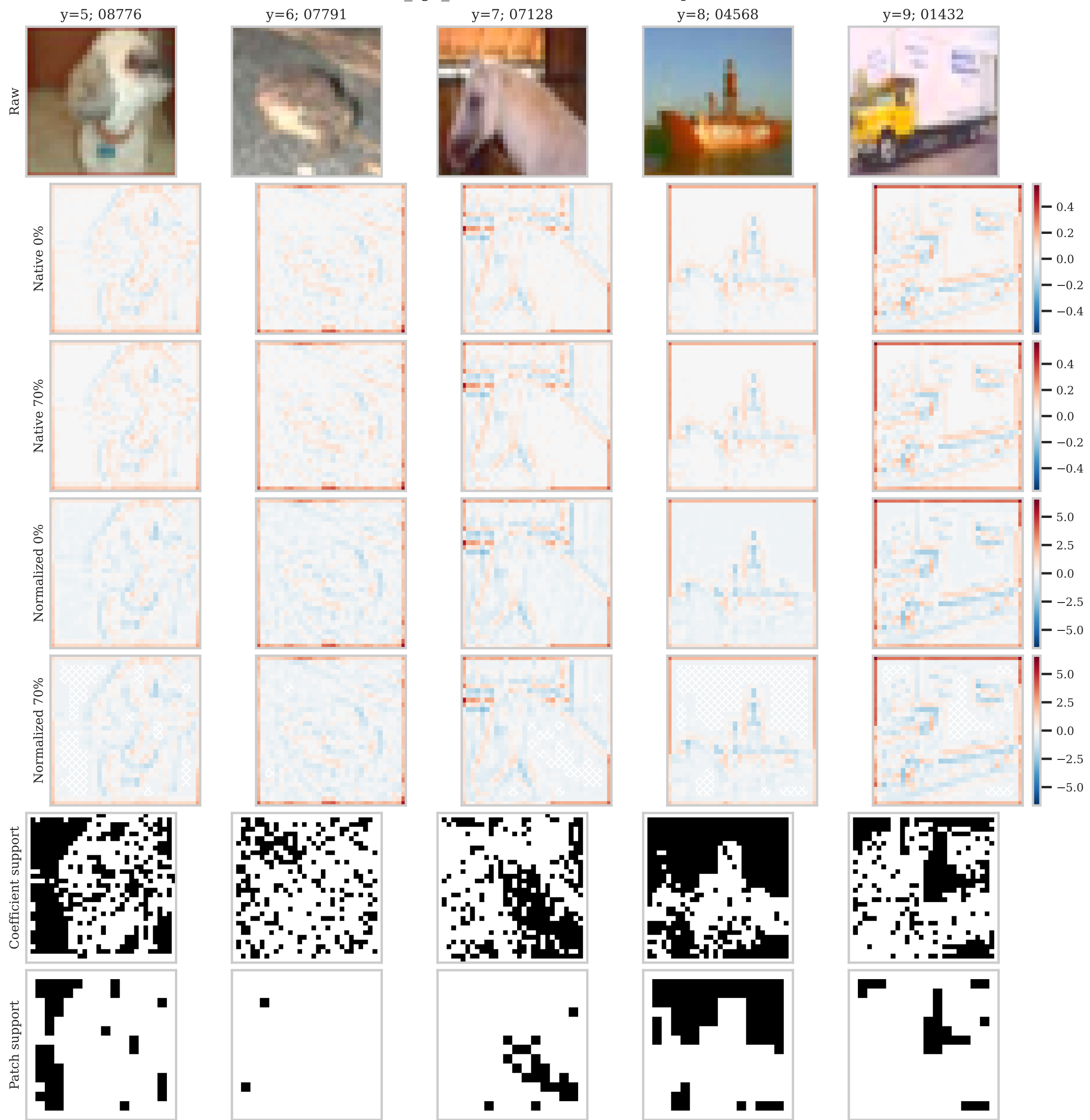
cifar10 | color_opponency | p70 | brightness 3 mean_rgb_contrast; hatched = absent patch
