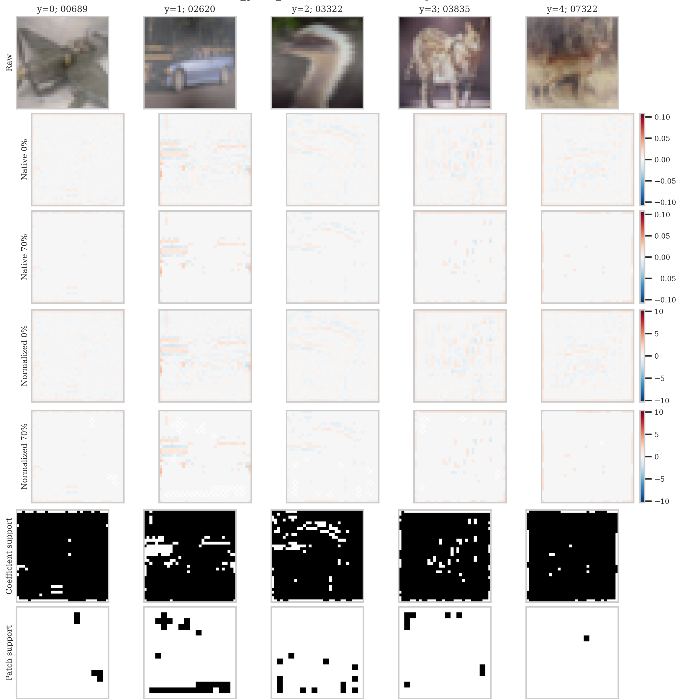
cifar10 | color_opponency | p70 | fog 3 red_green_contrast; hatched = absent patch
