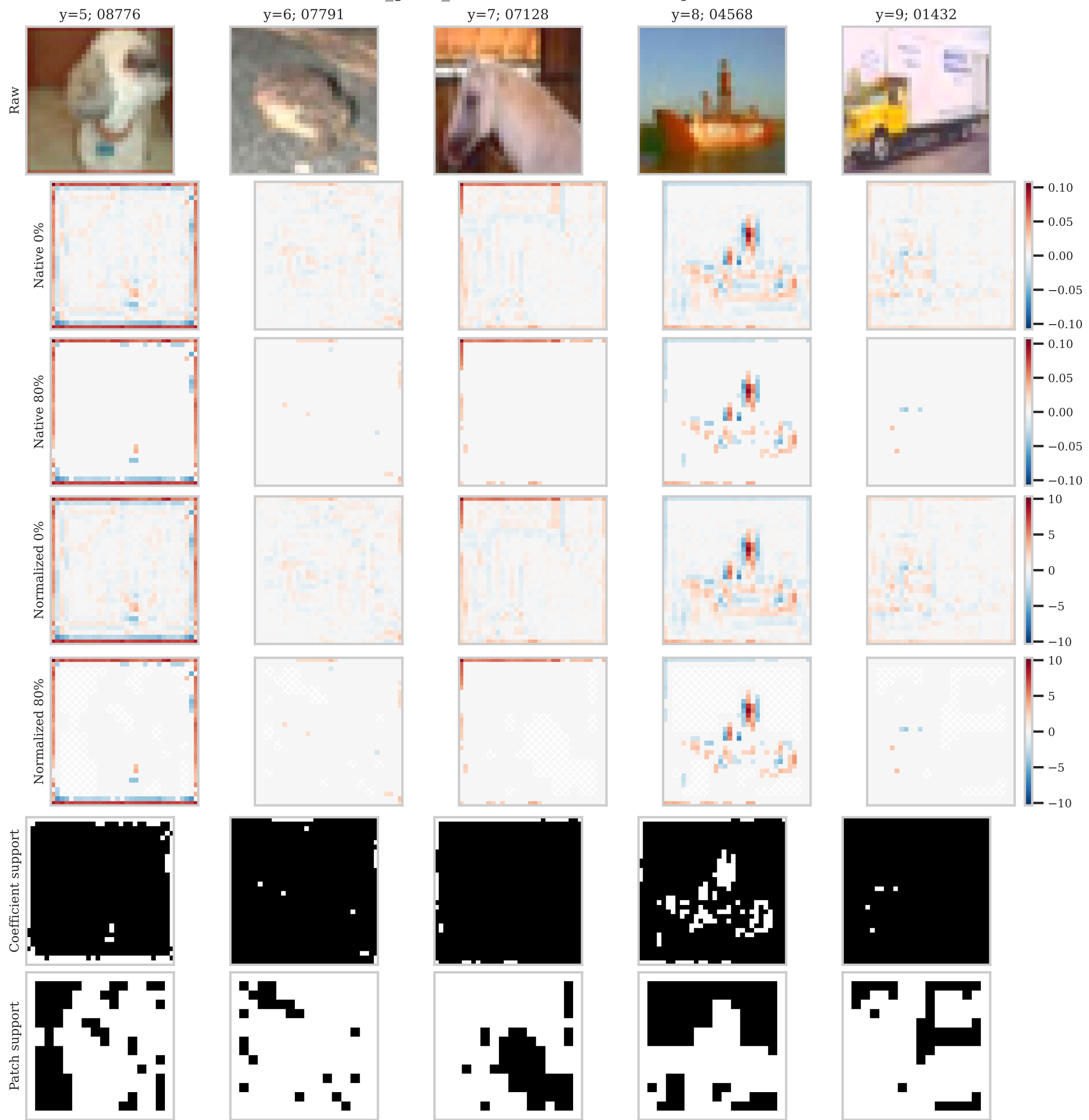
cifar10 | color_opponency | p80 | brightness 3 red_green_contrast; hatched = absent patch
