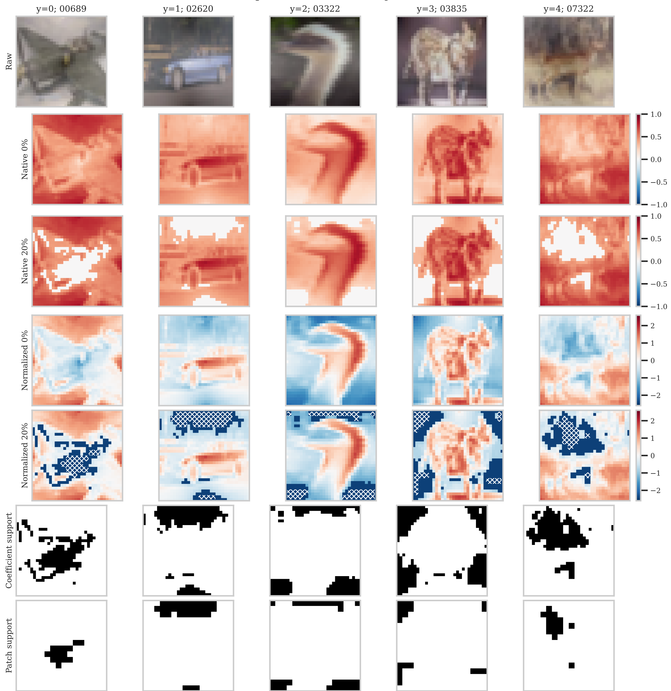
cifar10 | raw | p20 | fog 3 green; hatched = absent patch
