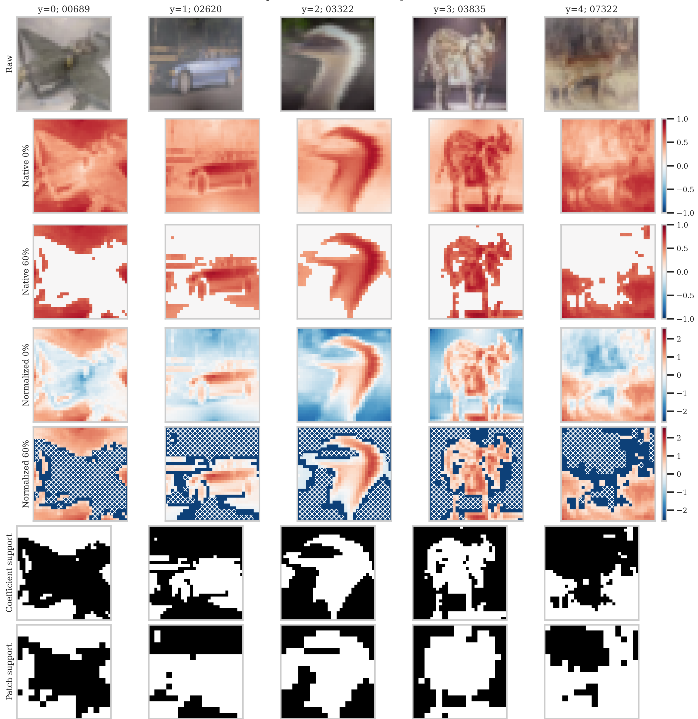
cifar10 | raw | p60 | fog 3 green; hatched = absent patch
