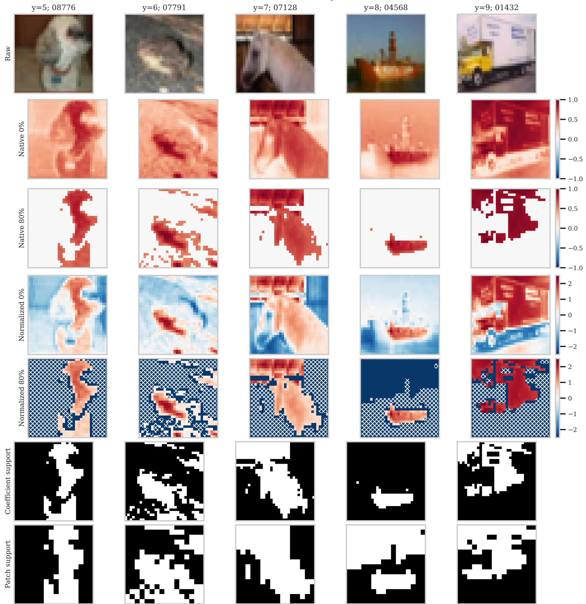
cifar10 | raw | p80 | clean test red; hatched = absent patch
