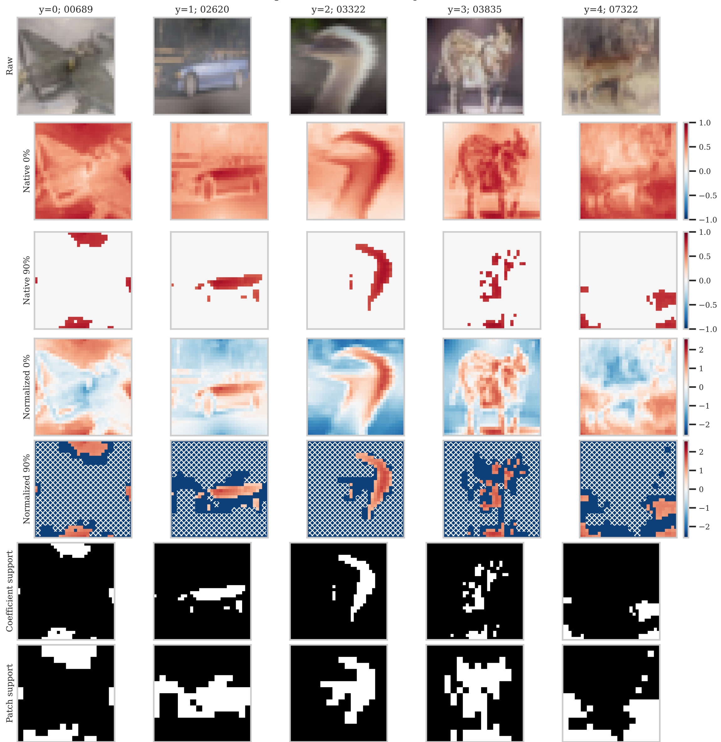
cifar10 | raw | p90 | fog 3 green; hatched = absent patch
