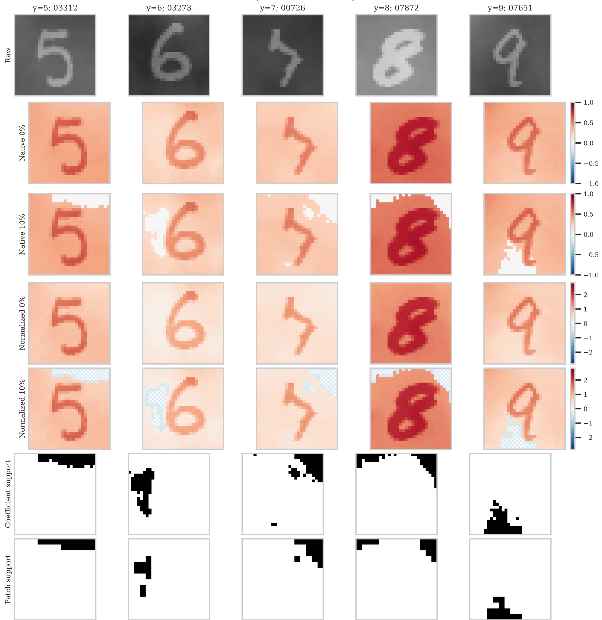
mnist | raw | p10 | fog fixed intensity; hatched = absent patch
