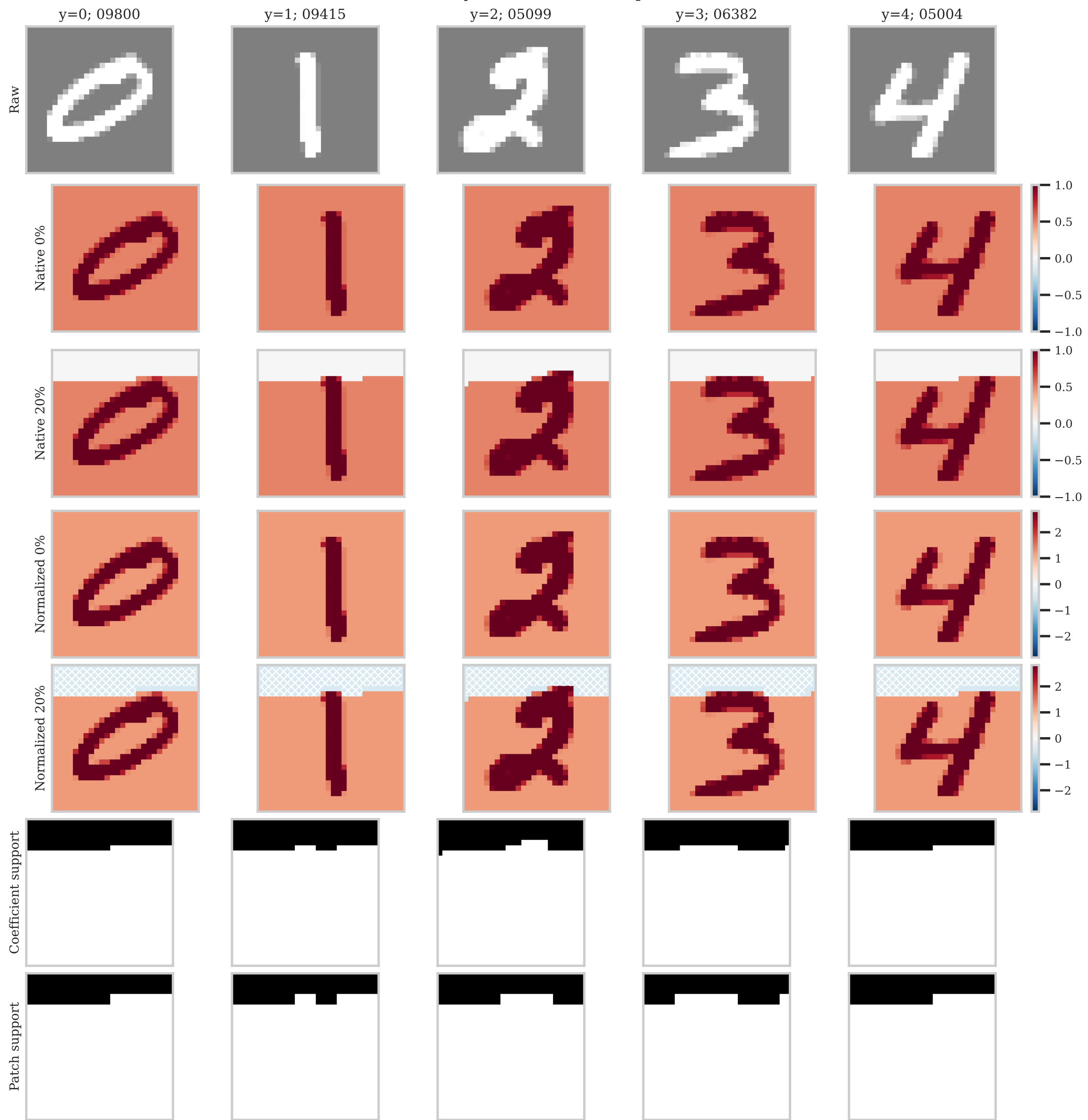
mnist | raw | p20 | brightness fixed intensity; hatched = absent patch
