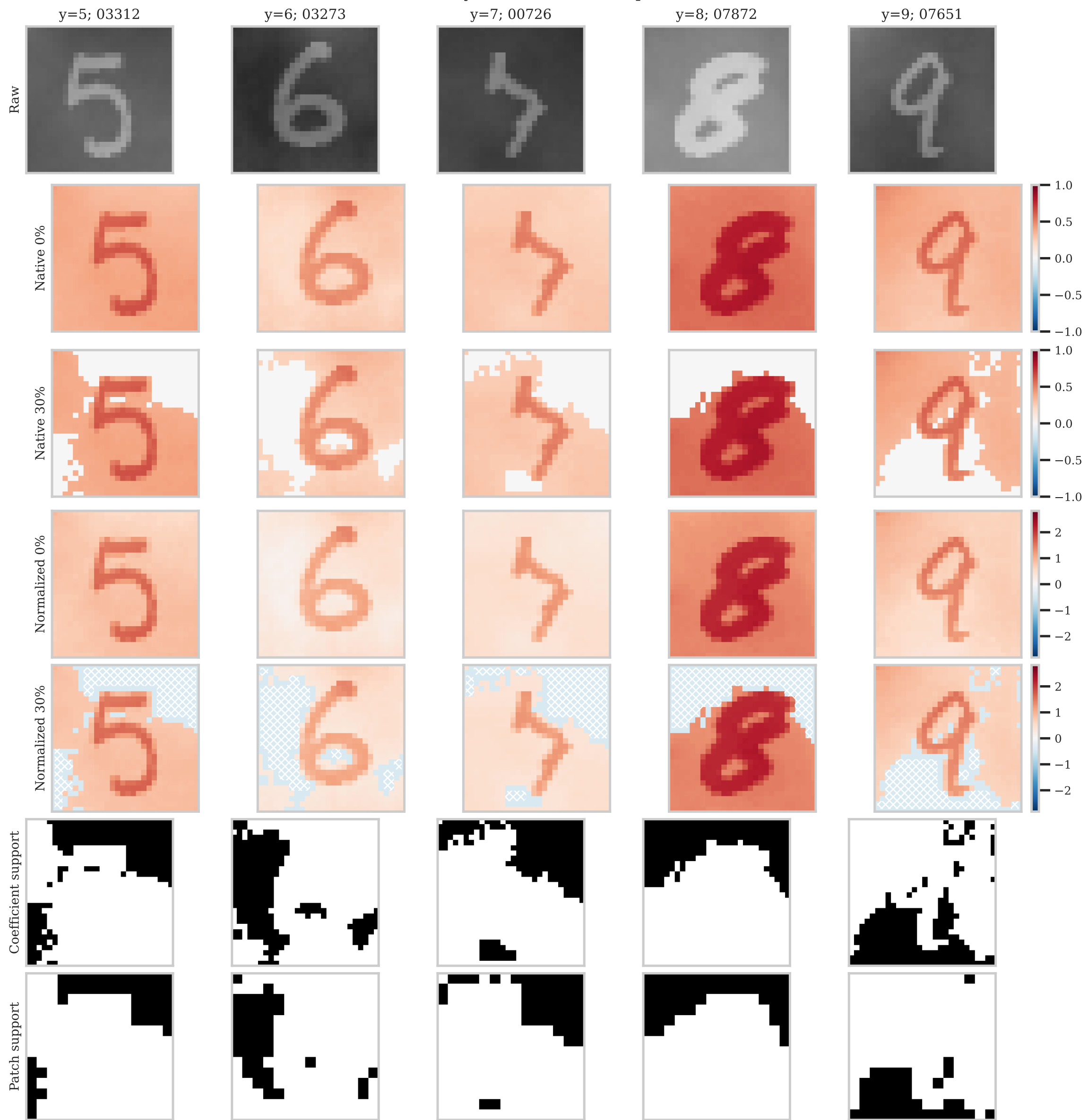
mnist | raw | p30 | fog fixed intensity; hatched = absent patch
