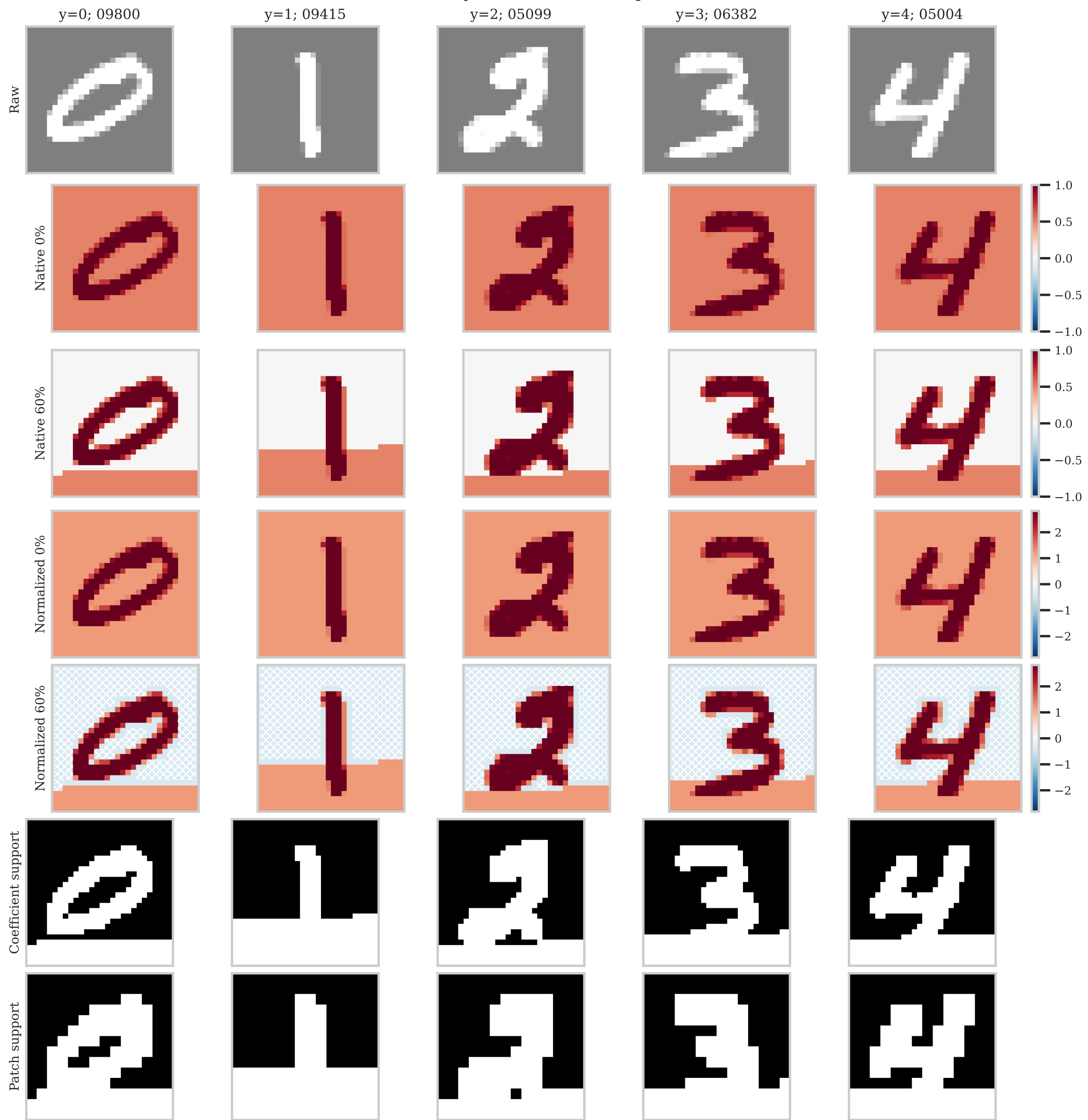
mnist | raw | p60 | brightness fixed intensity; hatched = absent patch
