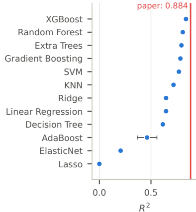
California Housing
