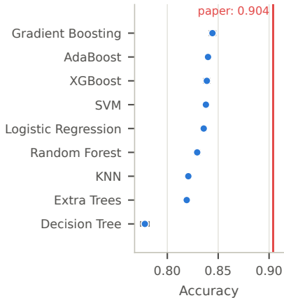
Adult
