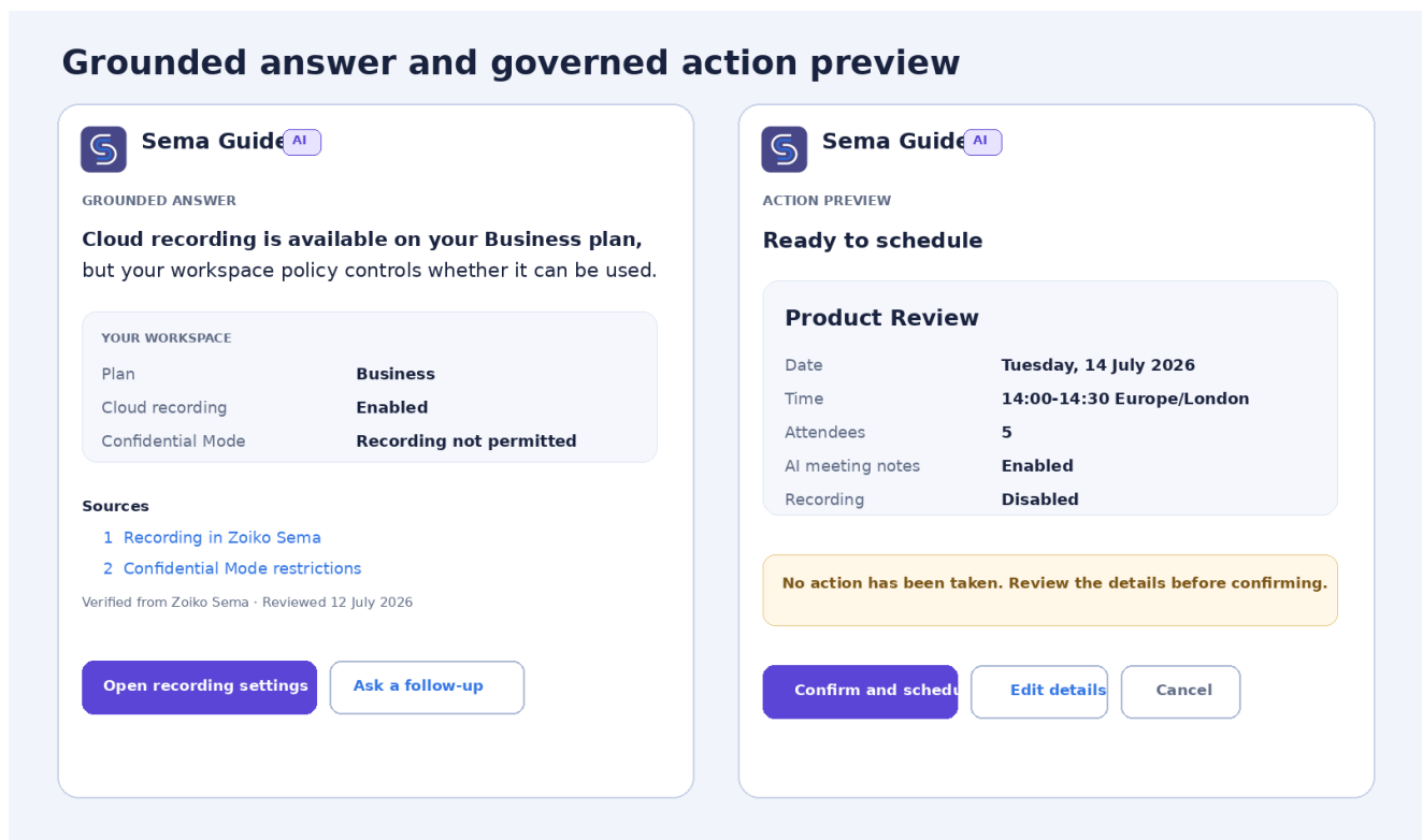
Figure 2. Verified answer and explicit action-preview patterns.
