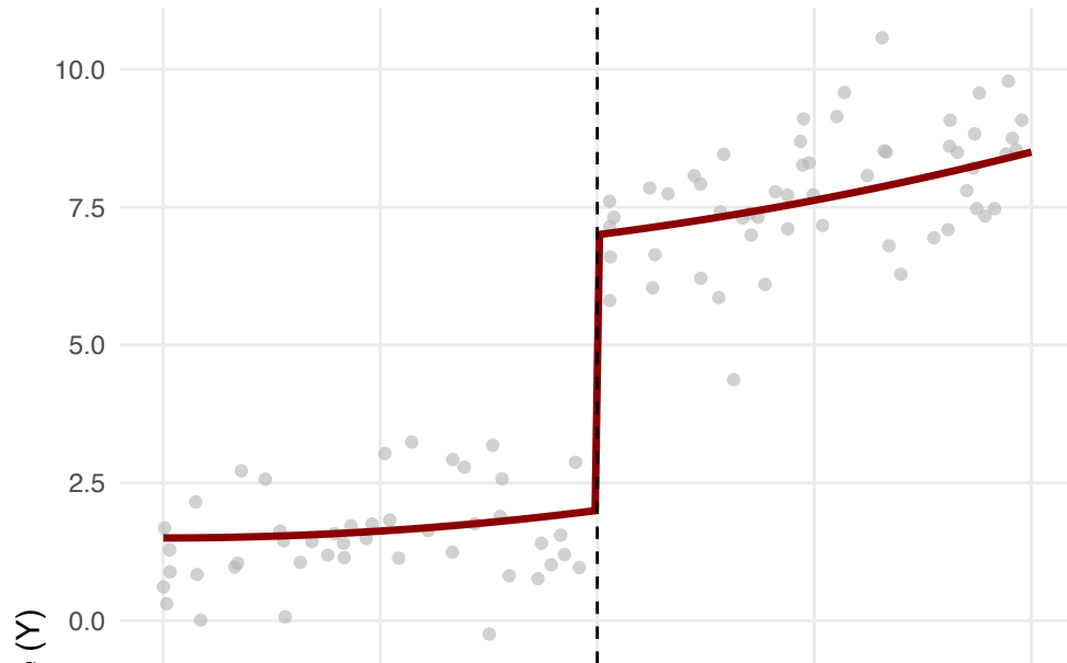
Case 3: Structural Break (Stress Test)
