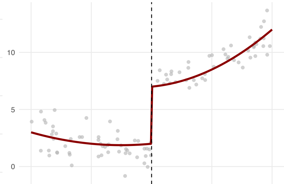
Case 4: Complex DGP (High Noise)
