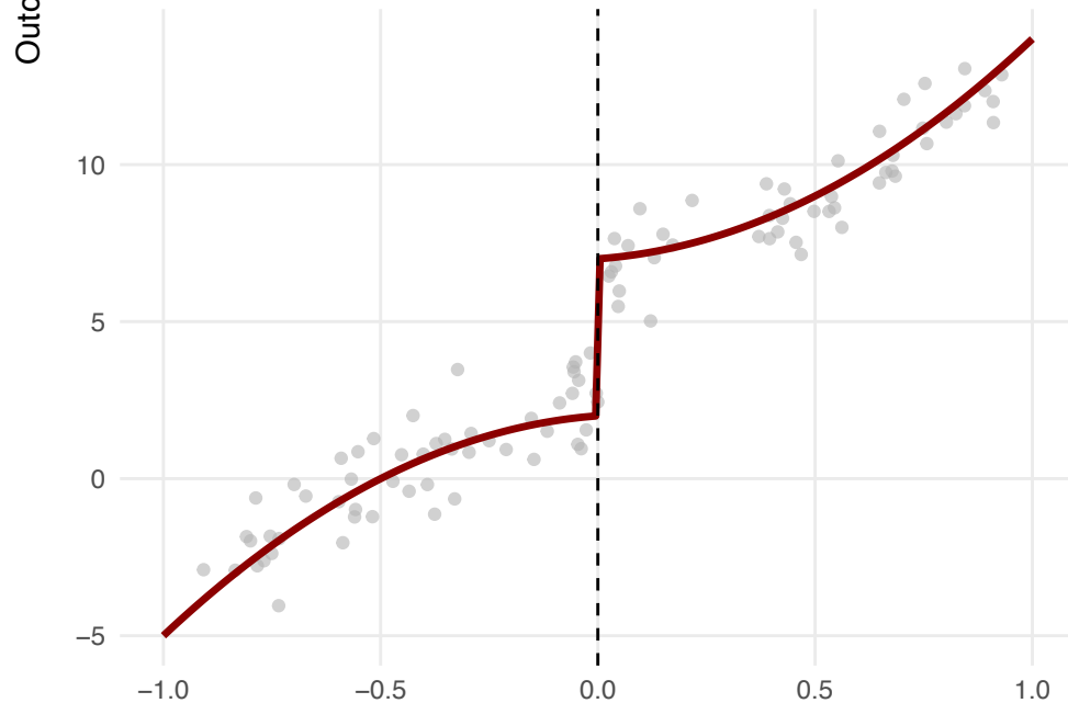
Case 3: Structural Break (Stress Test)
