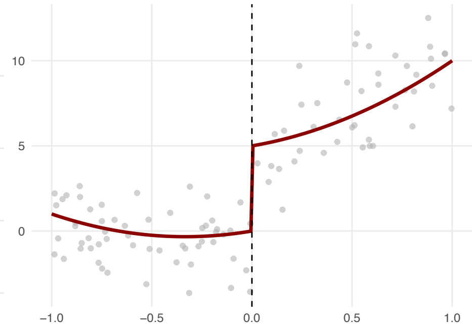
Case 4: Complex DGP (High Noise)
