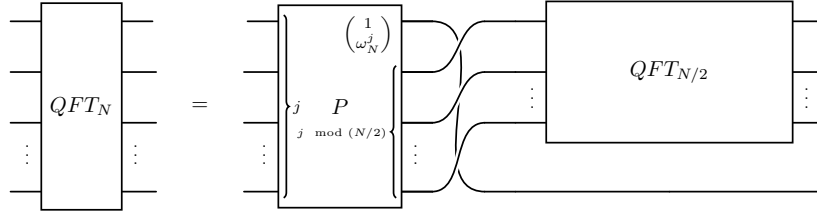
FIG. 3: Recursive definition of the quantum Fourier transform circuit, which shows how QFT_N can be defined in terms of QFT_{N/2} and some other simple operations. The circuit for the operation P is shown in Figure 2. This definition can be repeatedly applied to decompose the QFT_N operation into a quantum circuit. Note that the “base case” at which the decomposition is no longer needed is QFT_2 , which is equal to the Hadamard gate.
