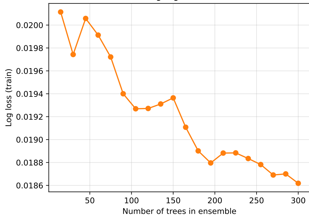
RF head — training log-loss vs. ensemble size
