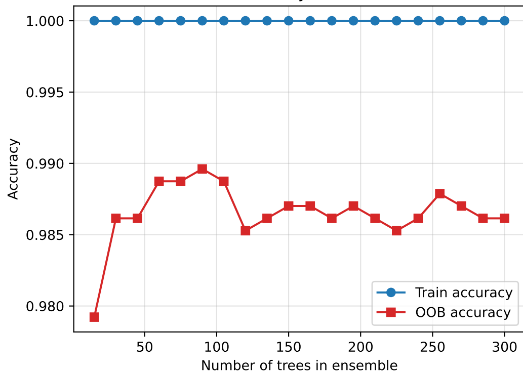
RF head — accuracy vs. ensemble size
