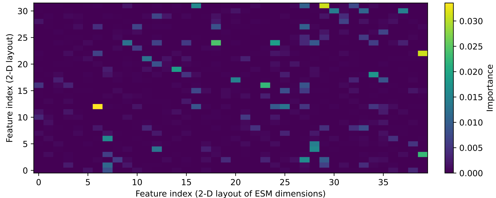
Random forest — normalised feature importances (embedding dims)
