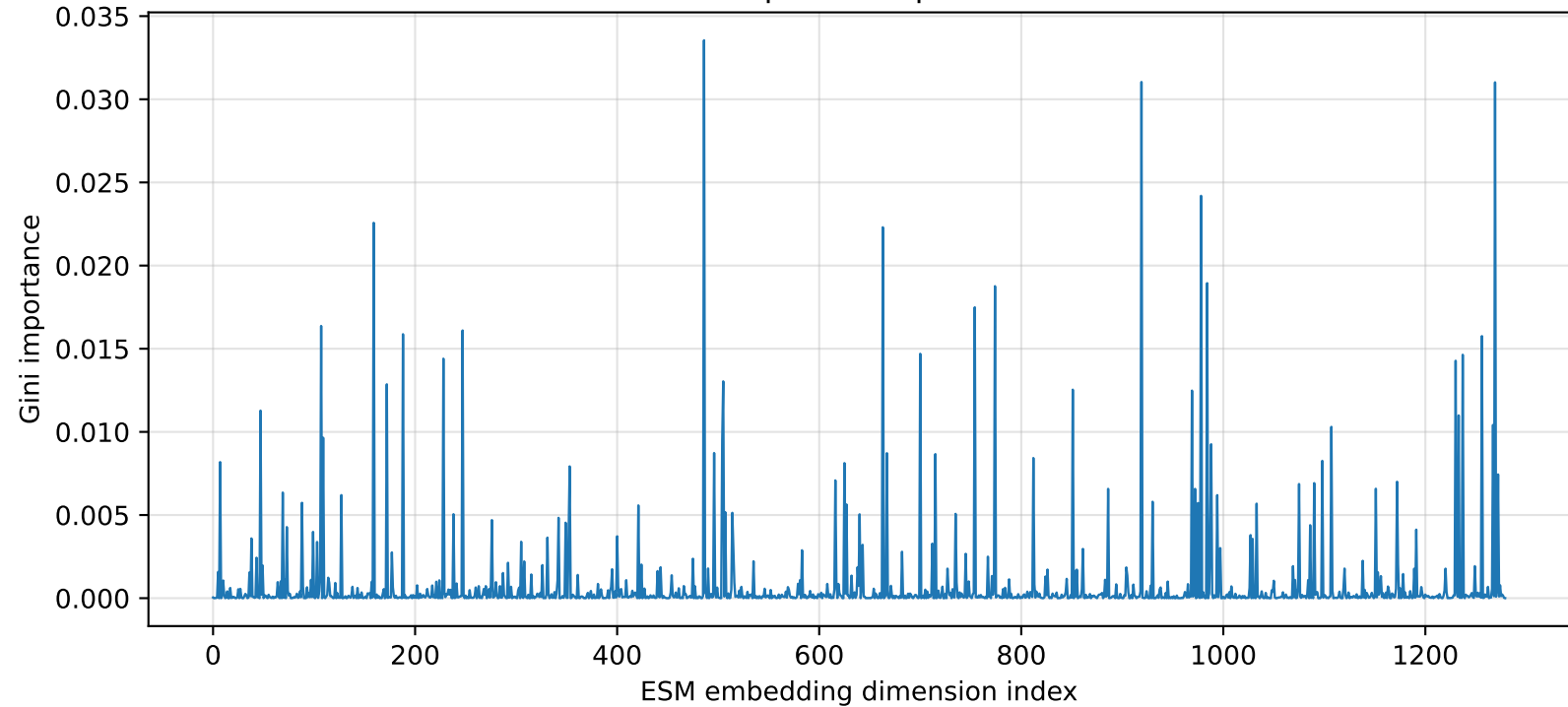
Random forest — importance profile across channels
