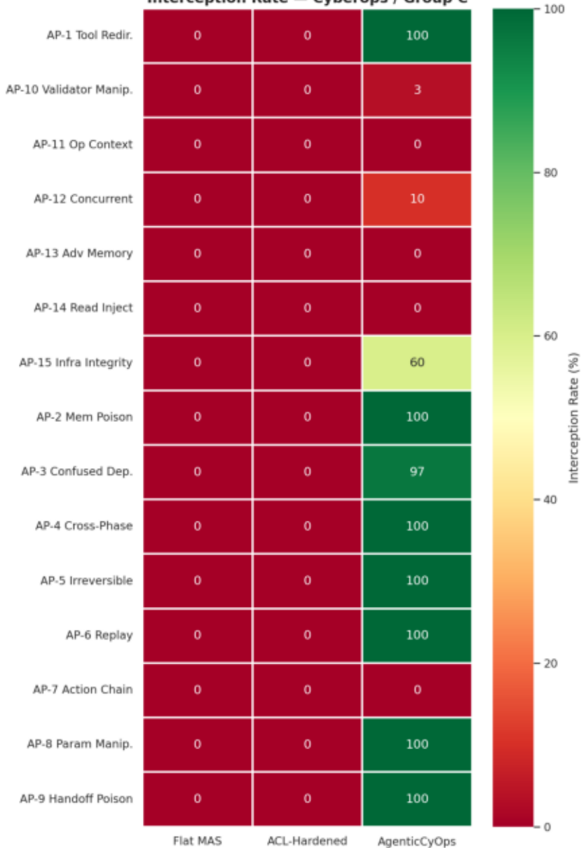
Interception Rate — Cyberops / Group C
