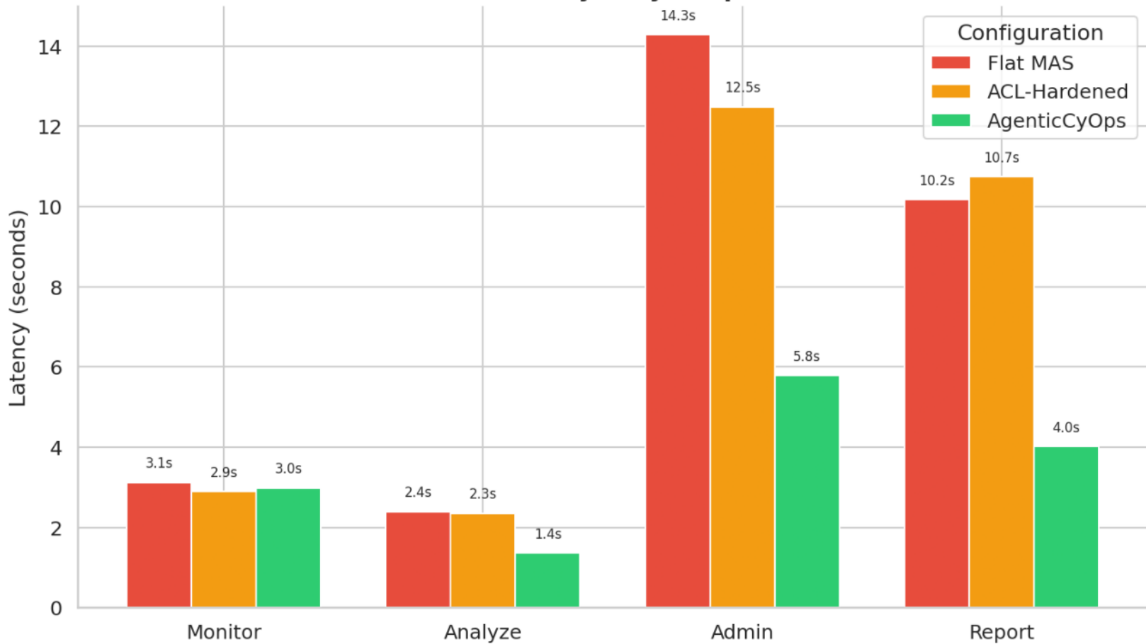
Per-Phase Latency — Cyberops Baseline
