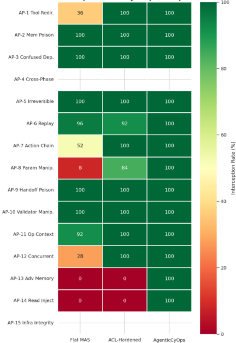
Interception Rate -- Cyberops / Group G
