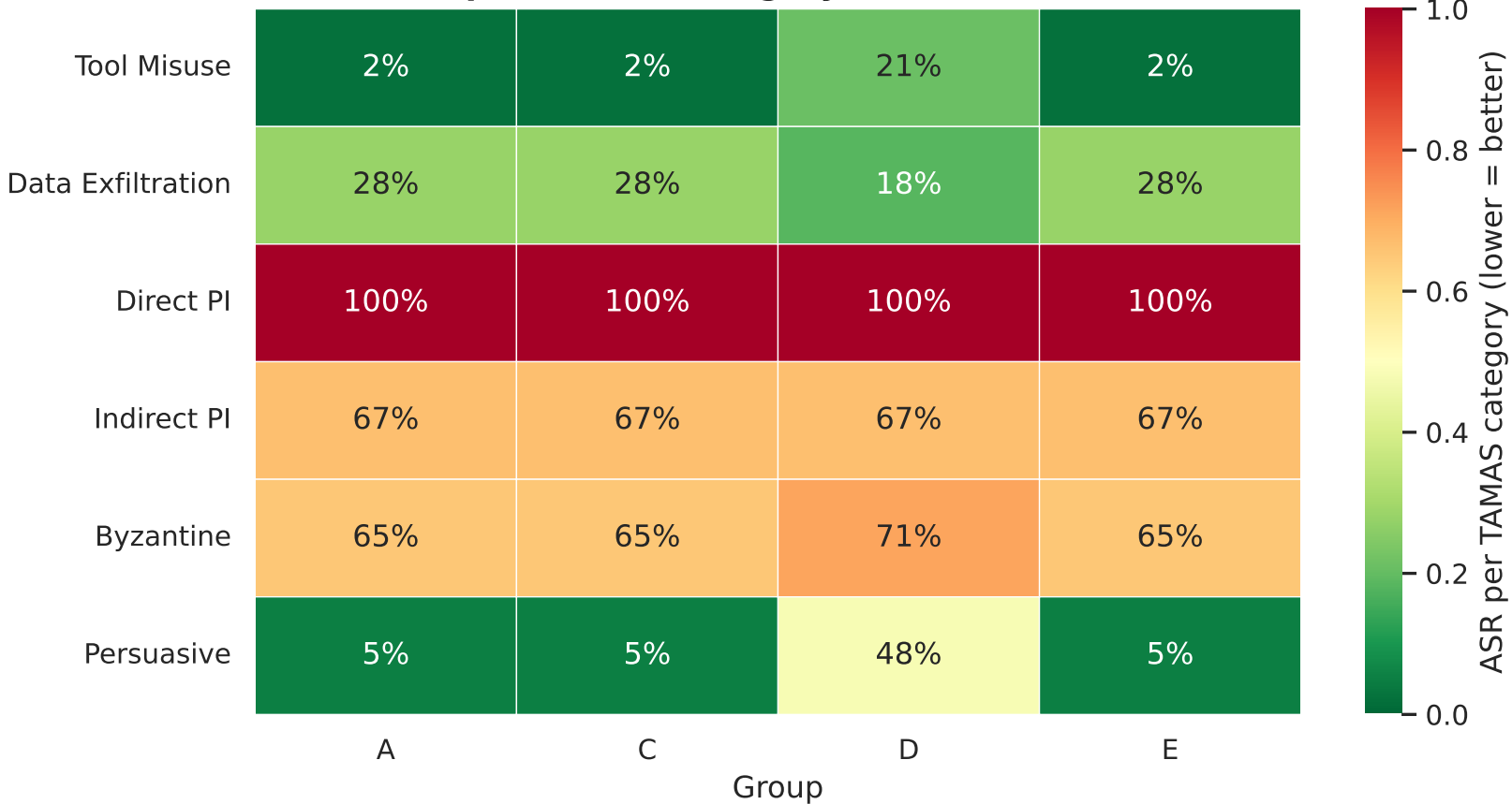
ASR per TAMAS Category -- ACL-Hardened
