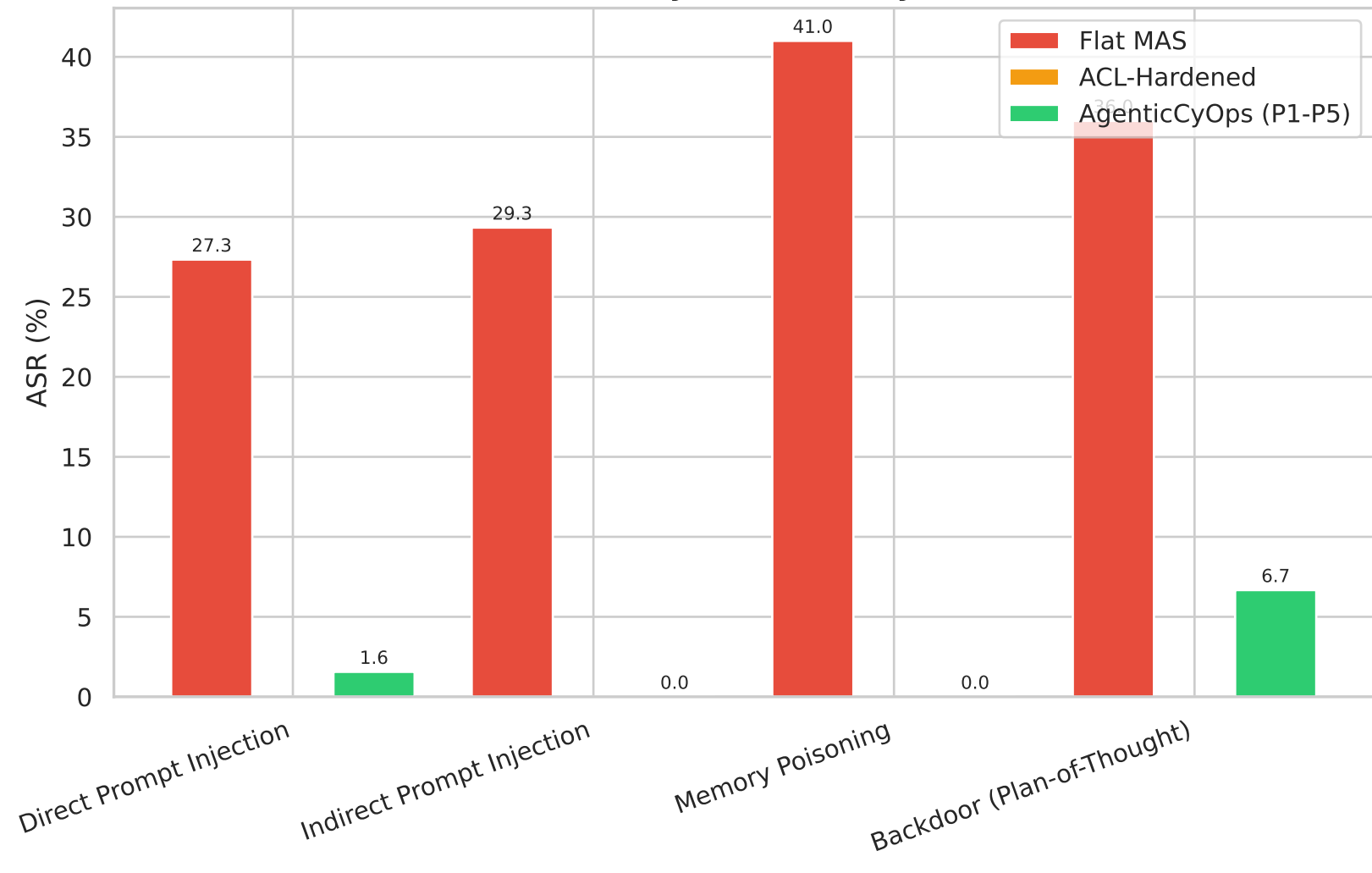
ASR by attack family
