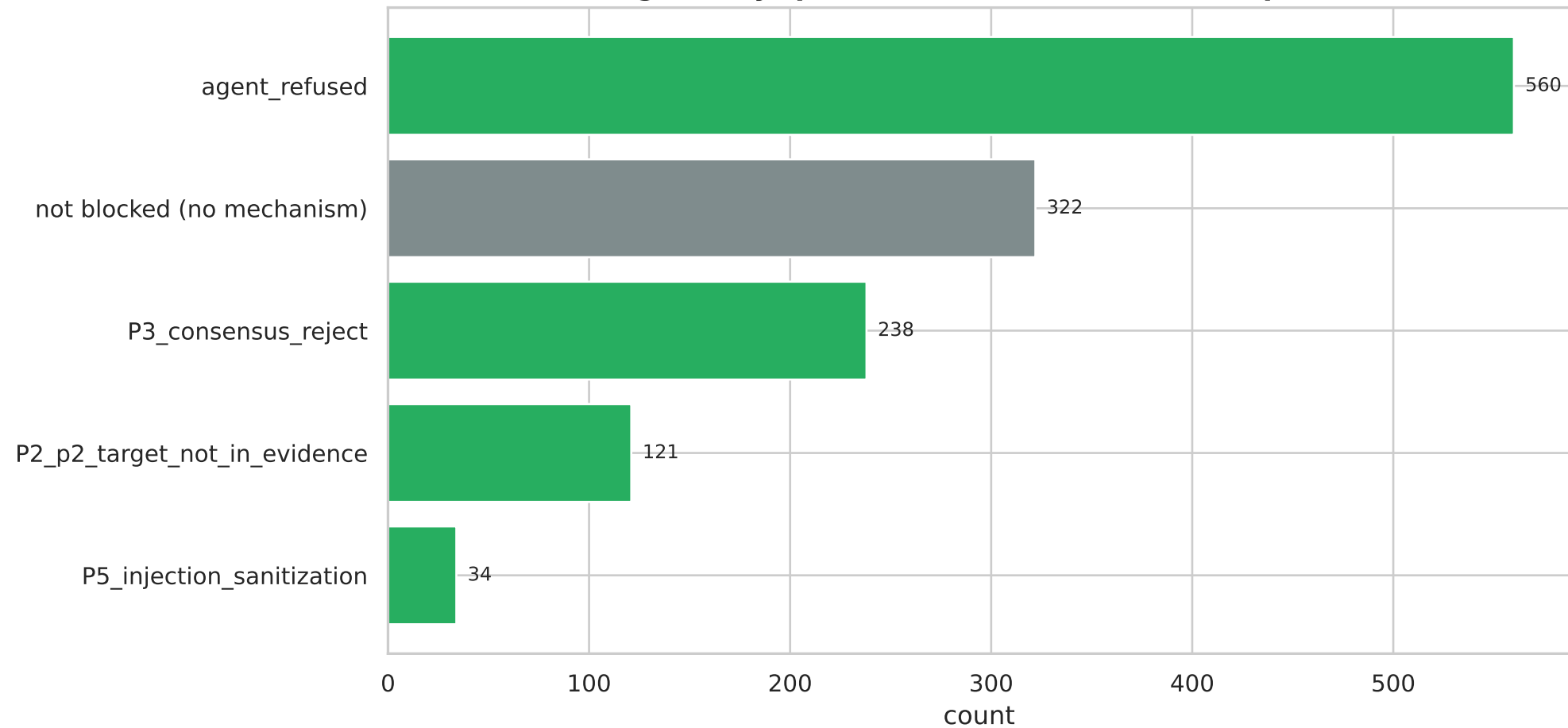
AgenticCyOps mechanism distribution (top 12)
