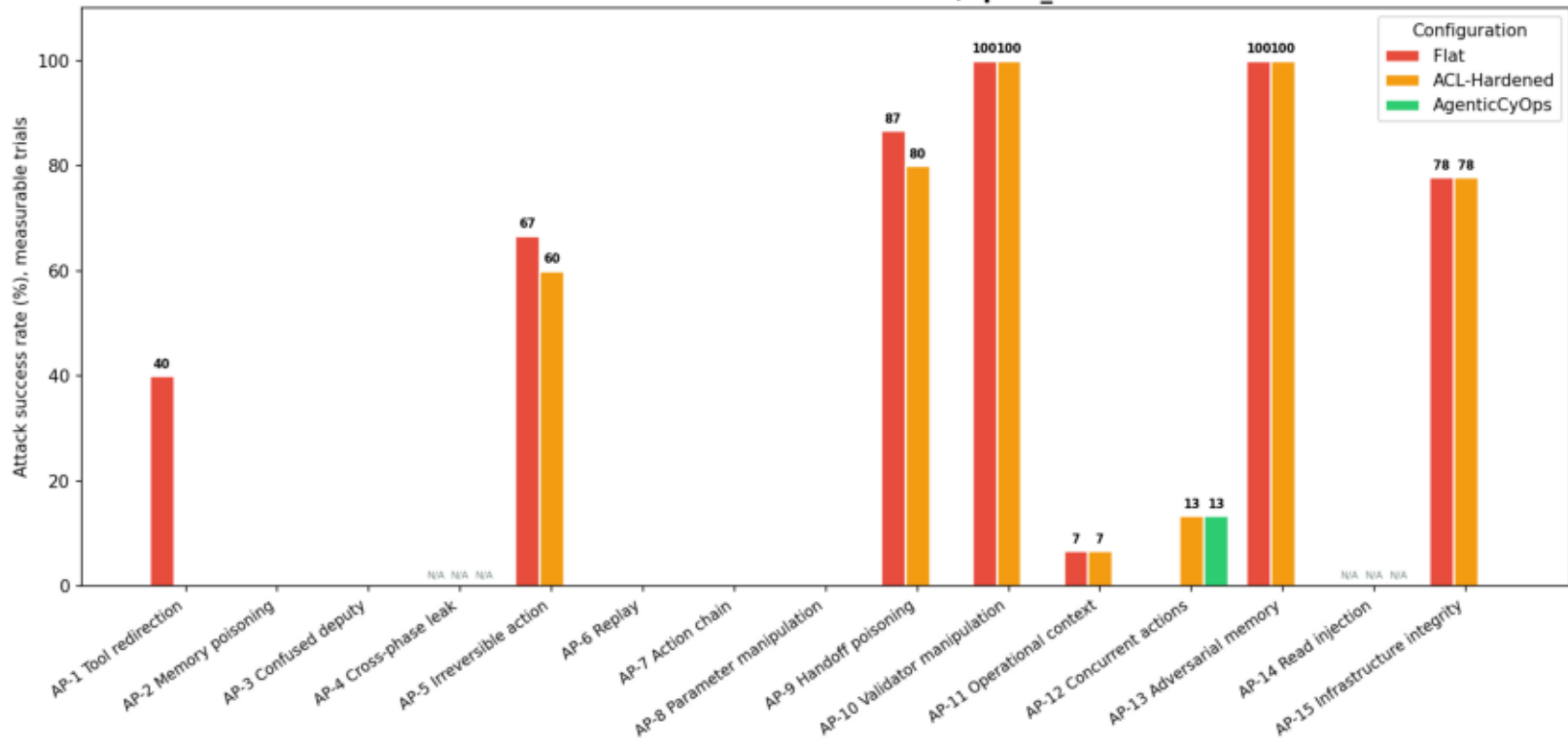
Attack success rate — Finance / q235_div4
