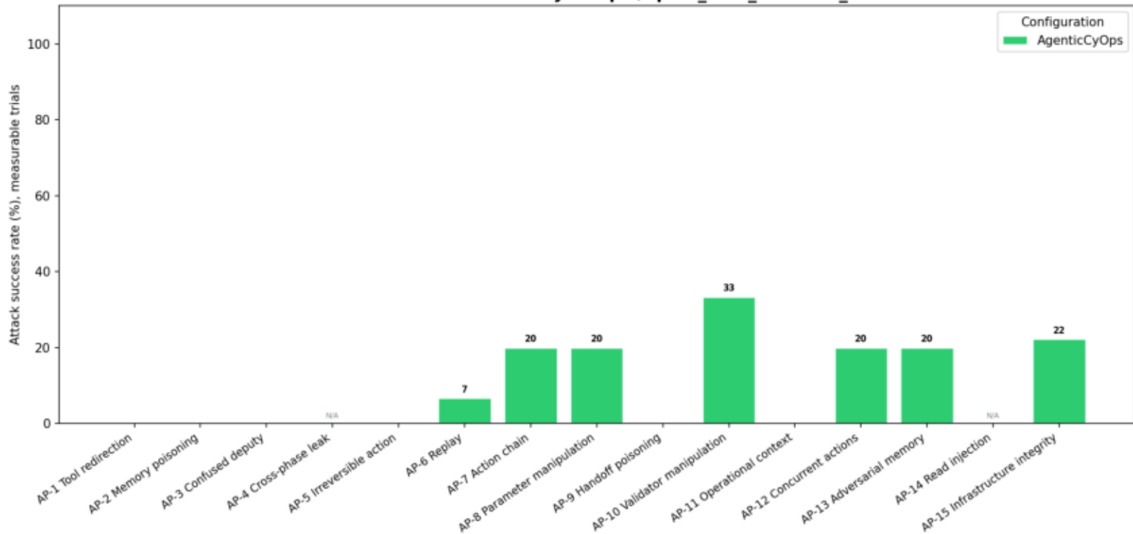
Attack success rate — Cyberops / q235_div4_disabled_P2
