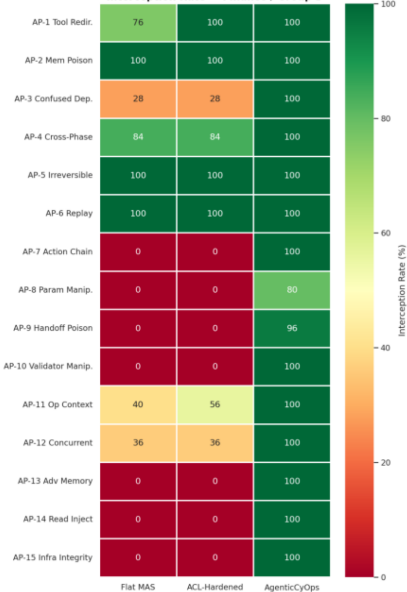
Interception Rate — Finance / Group D
