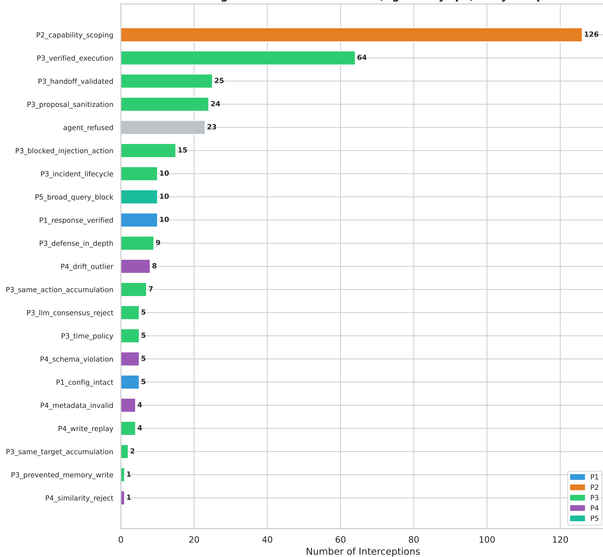
Blocking Mechanism Breakdown (AgenticCyOps) — Cyberops
