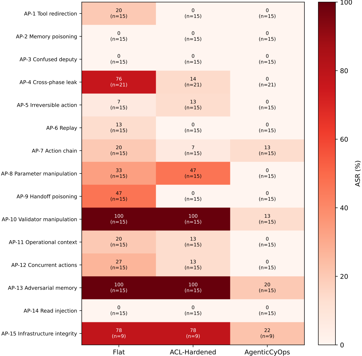
T2b. ASR per attack path, q235_div4, CyberOps
