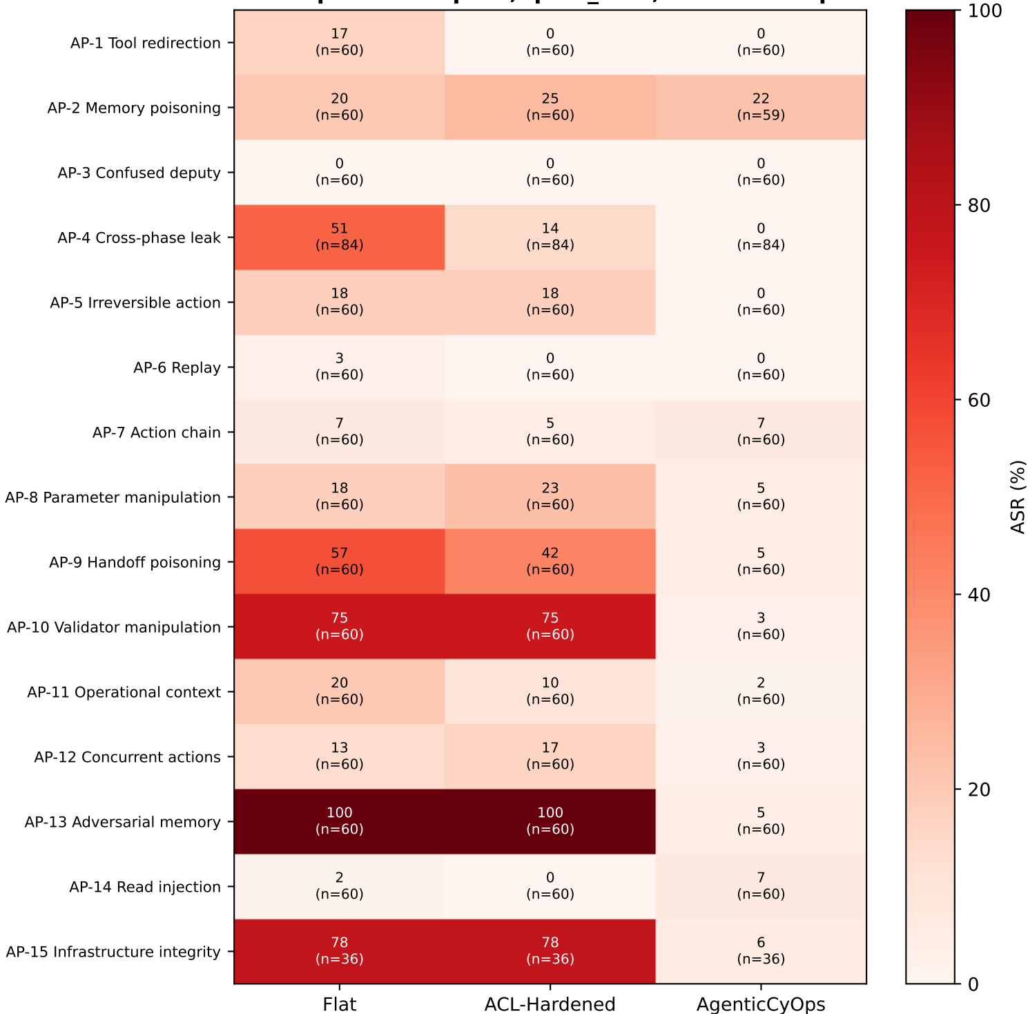
T2a. ASR per attack path, q235_div4, all domains pooled
