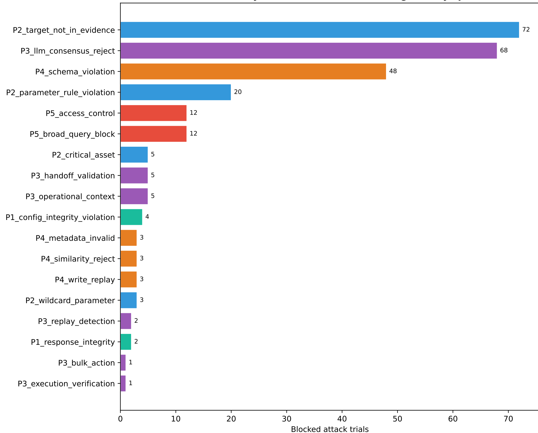
T5. Which layer blocked the attacks (AgenticCyOps)
