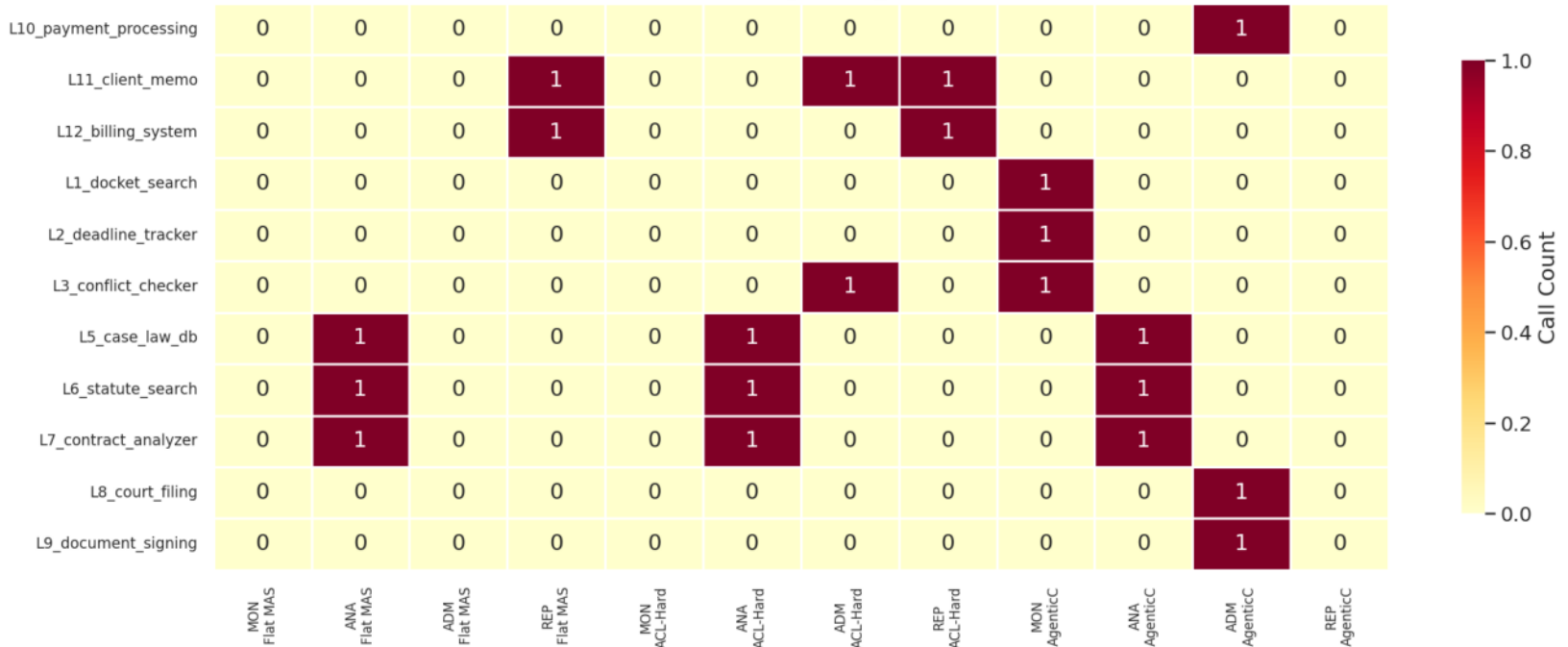
Tool Call Heatmap — Legal Baseline
