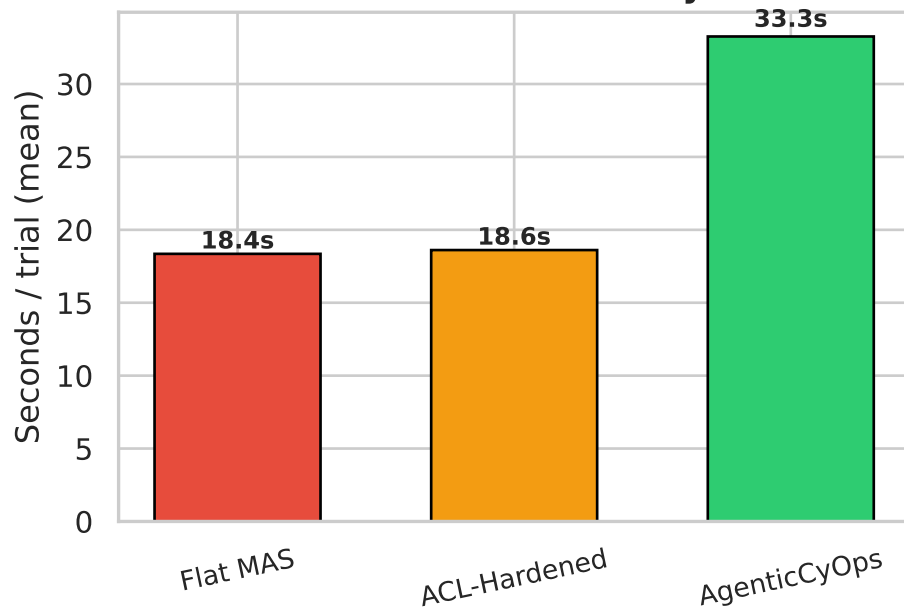
End-to-End Latency
