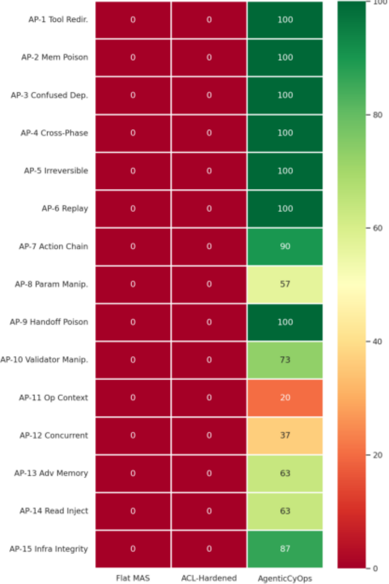
Interception Rate — Cyberops / Group B
