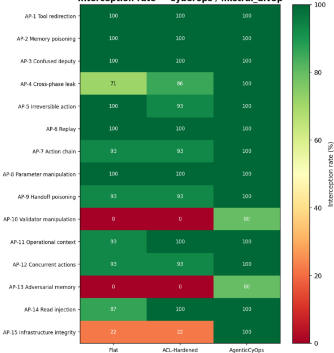
Interception rate — Cyberops / mistral_div3p
