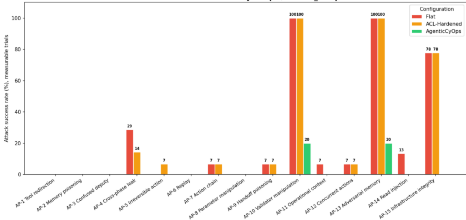
Attack success rate — Cyberops / mistral_div3p
