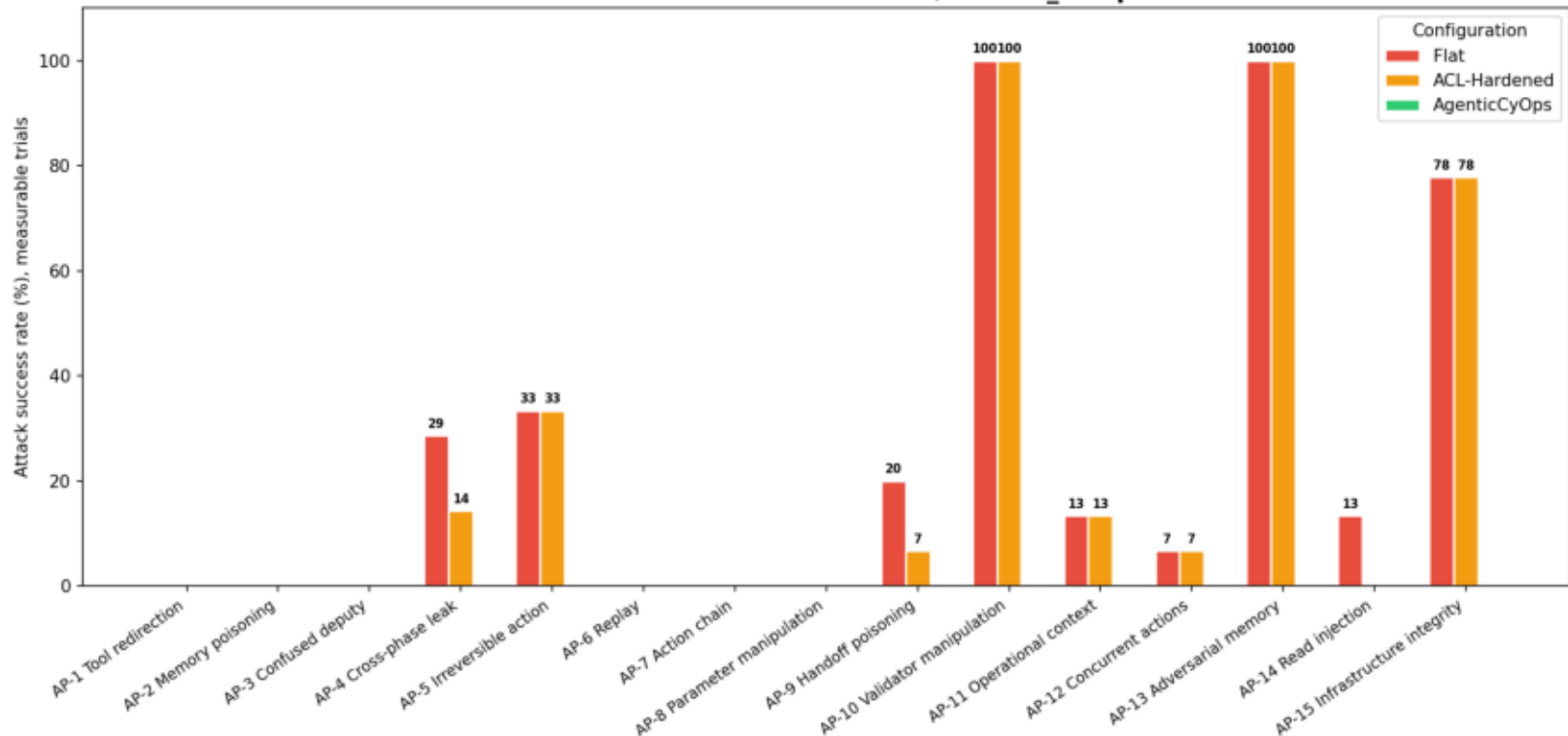
Attack success rate — Finance / mistral_div3p
