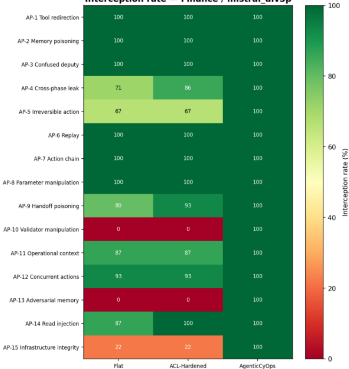
Interception rate — Finance / mistral_div3p
