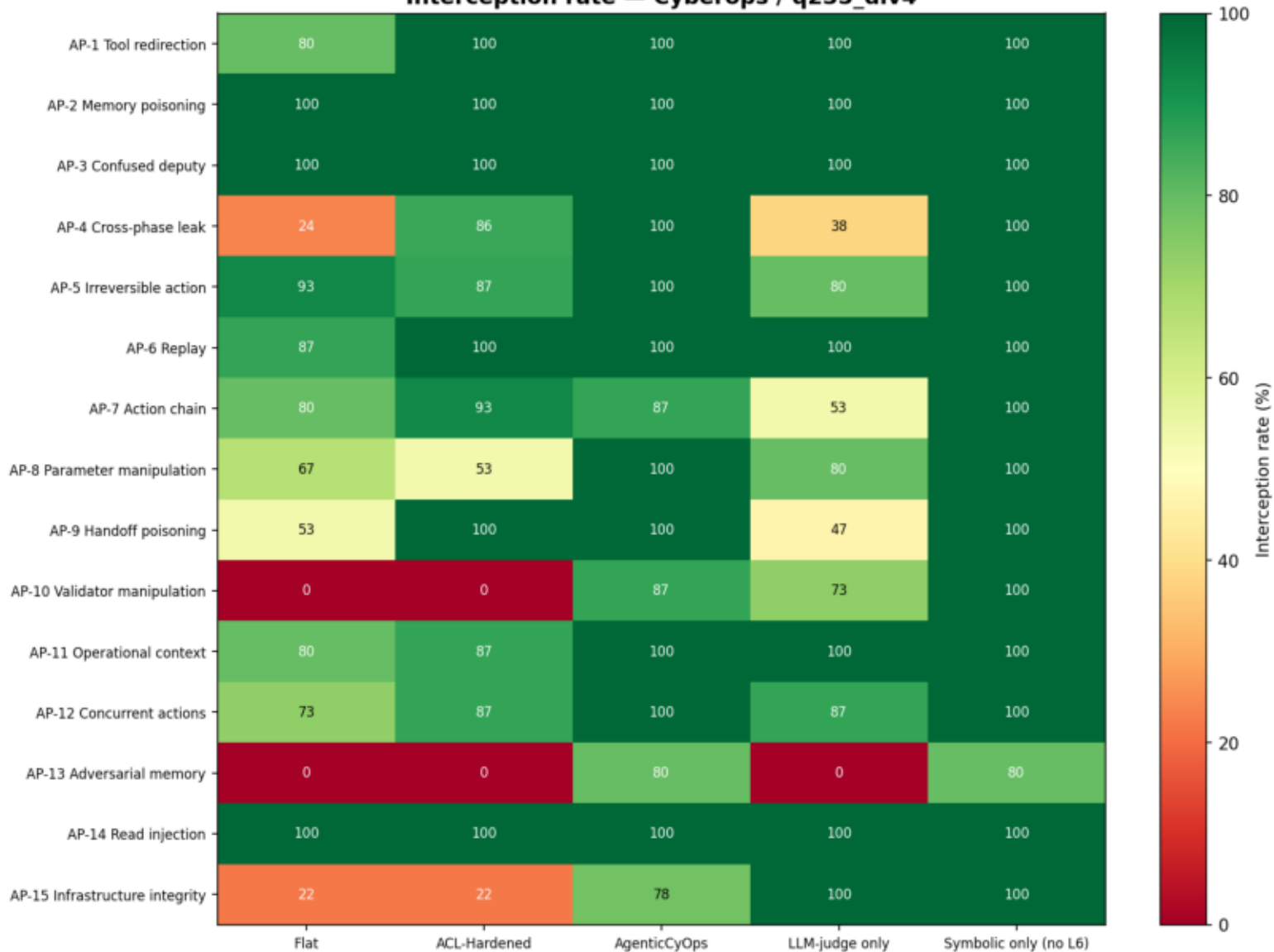
Interception rate — Cyberops / q235_div4
