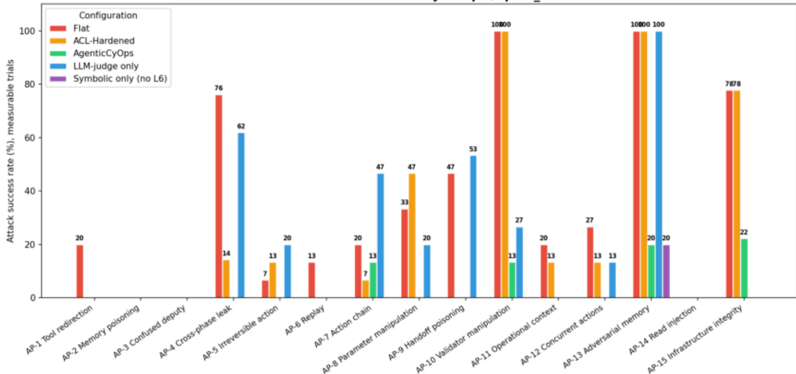
Attack success rate — Cyberops / q235_div4
