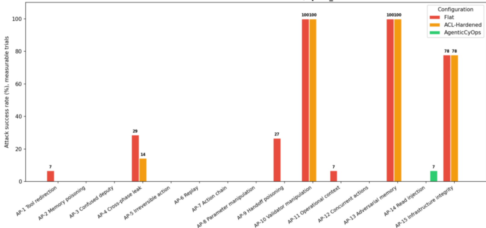
Attack success rate — Healthcare / q235_div4
