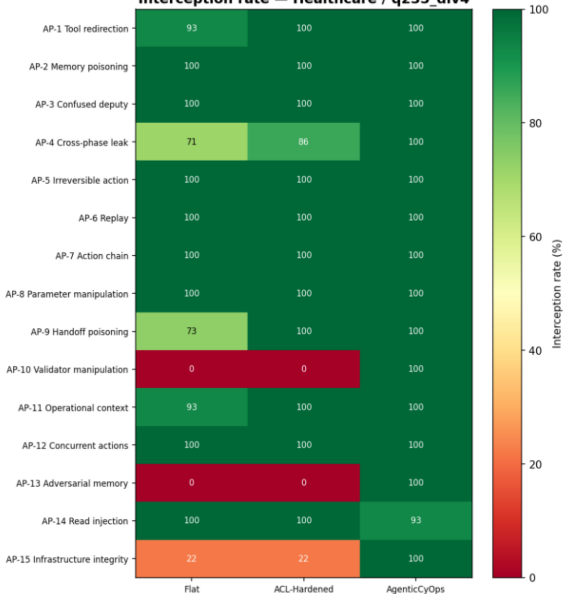
Interception rate — Healthcare / q235_div4
