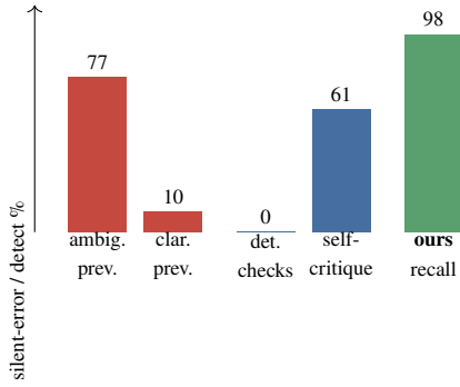
Figure 1: Silent-error prevalence (red: ambiguous 77% vs. clarified 10%) and detection recall (blue baselines vs. our contracts, green). Deterministic checks detect 0%; self-critique’s 61% comes with 40% false-positives.
