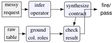
Figure 3: End-to-end pipeline. From only a messy request and a raw table, the system infers the operator (98%), grounds column roles (74–83%), synthesizes the contract (78%), and checks the result—nothing structured is provided.
