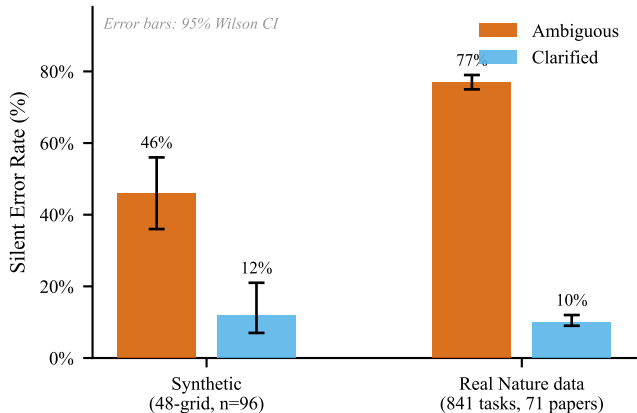
Fig. 1 — Silent Error Rate: Ambiguous vs. Clarified Prompts
