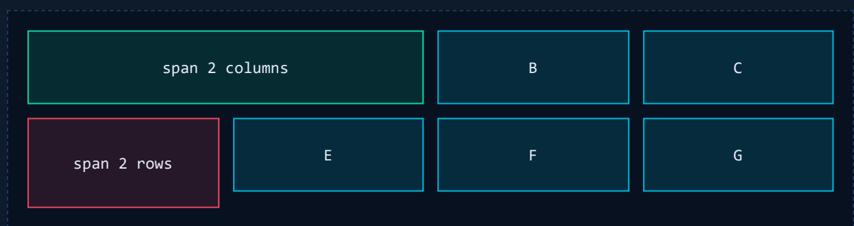
SPANNING GRAPH
