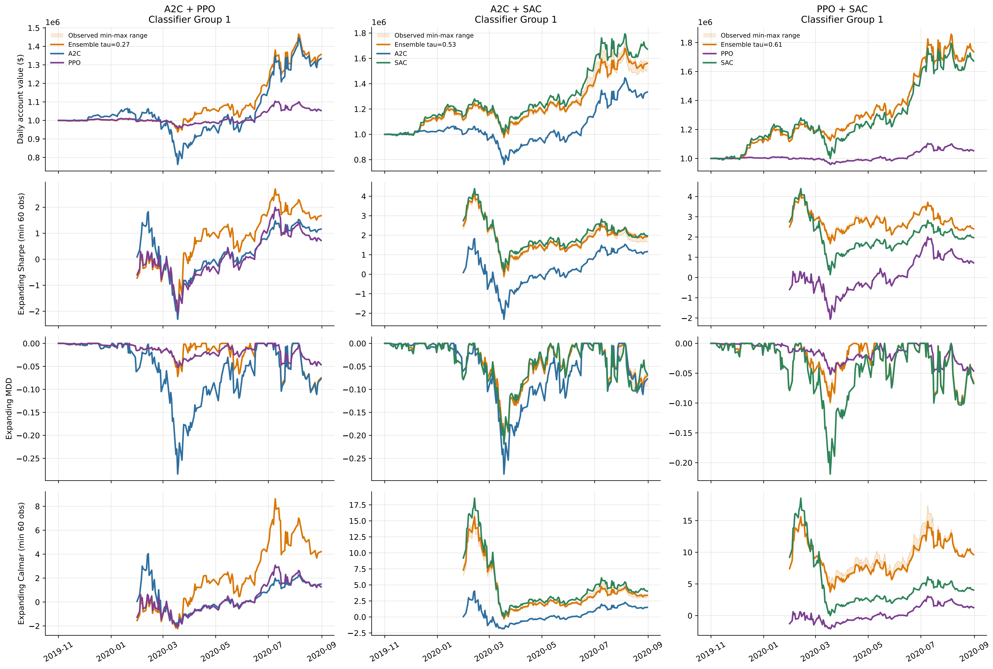
Figure 3: HSTech10 Performance Across 30 Classifier Refits
