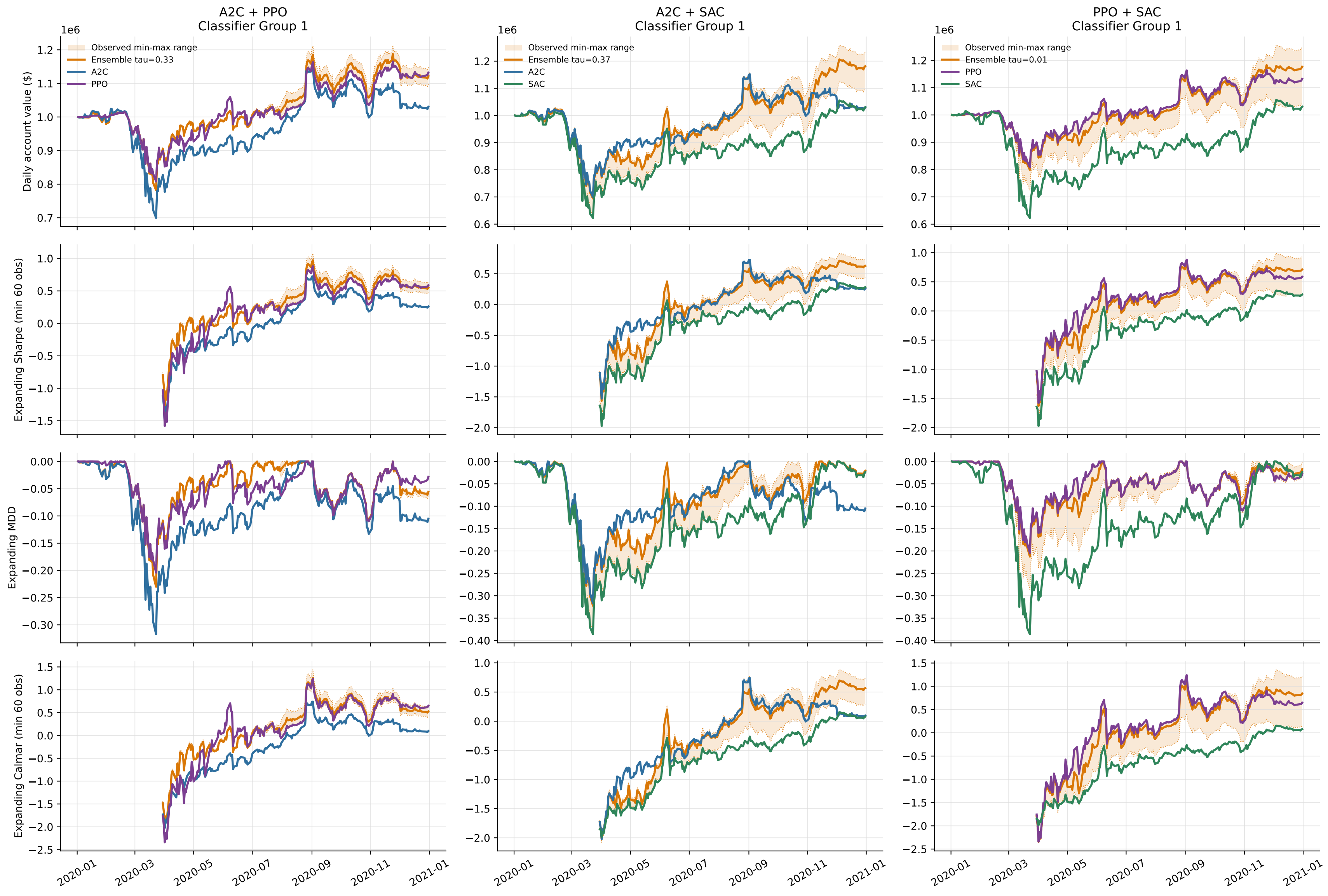
Figure 3: DJ30 Performance Across 30 Classifier Refits
