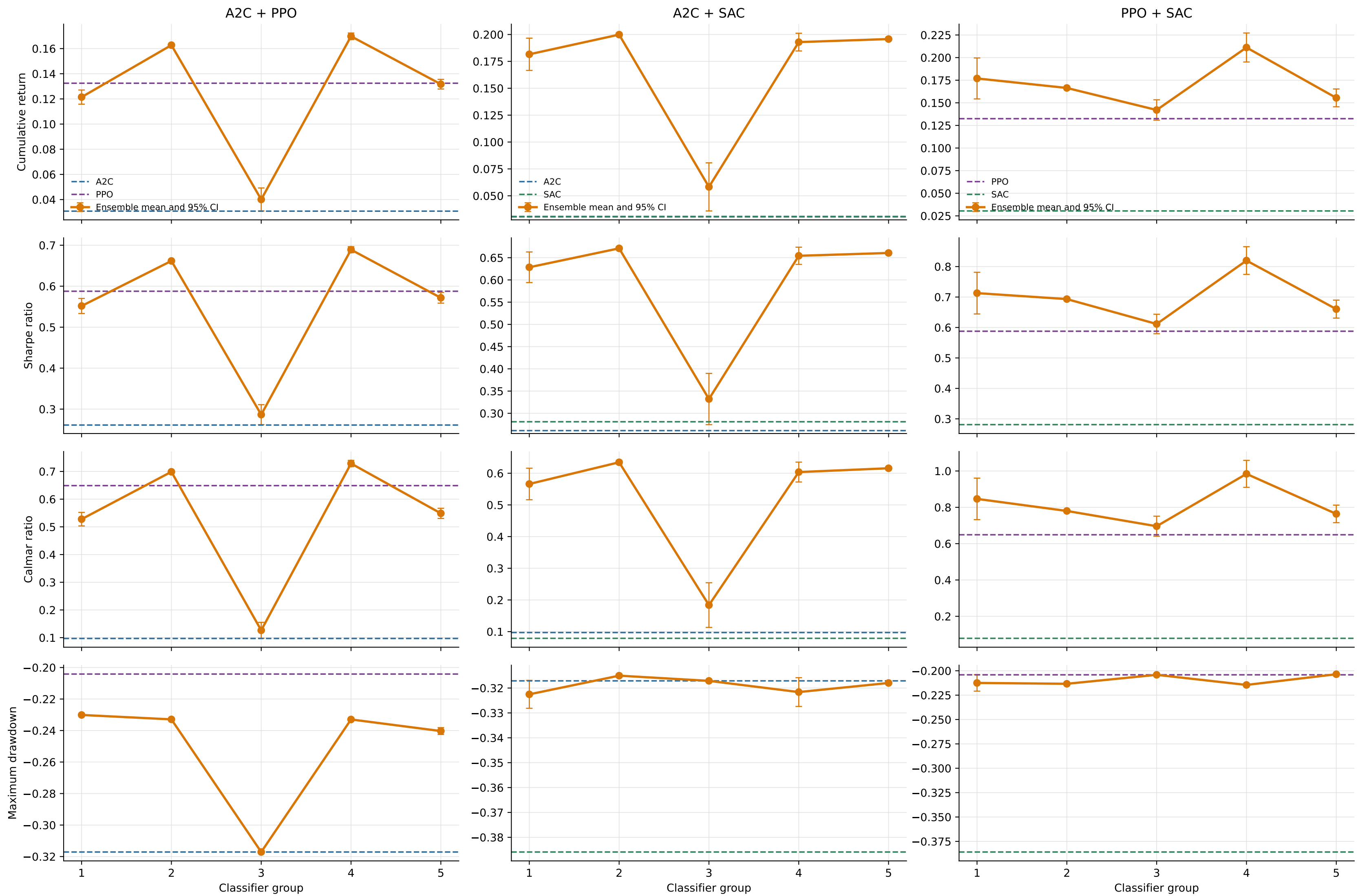
Figure 4: Classifier-Group Comparison Across 30 Classifier Refits
