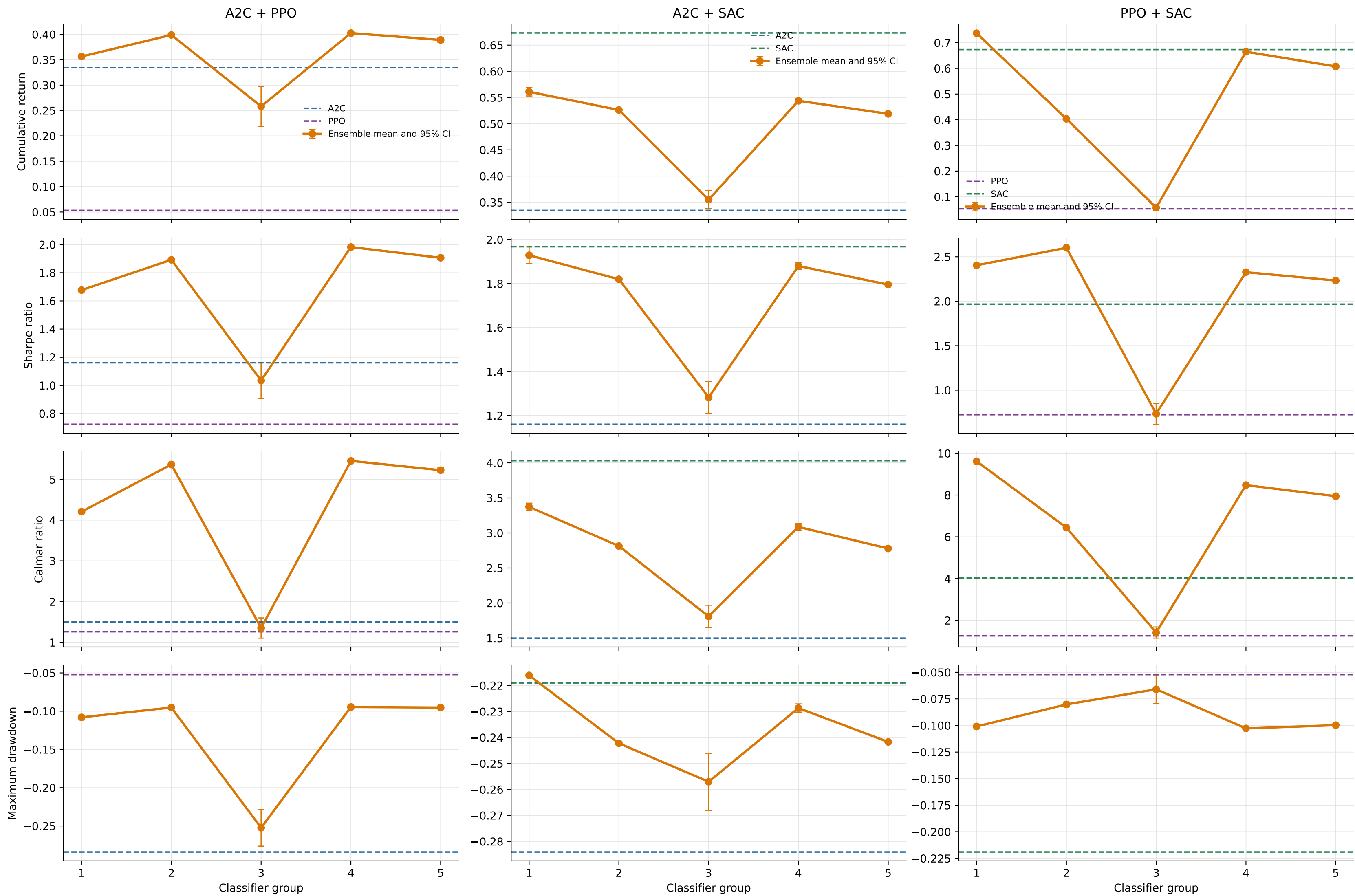
Figure 4: HSTech10 Classifier-Group Comparison
