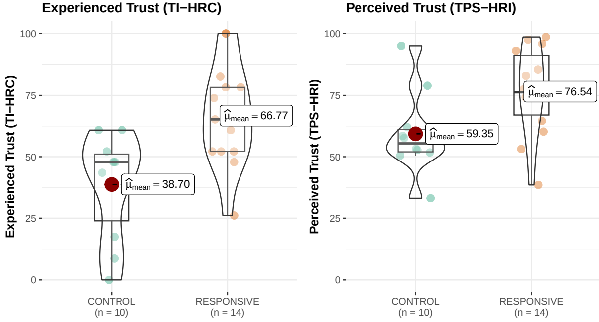
Figure 3: Distribution of Trust Perception by interaction policy. Points represent individual observations; violins depict score distributions. Red points indicate group means with 95% confidence intervals. Statistical comparisons are reported in the Results section.
